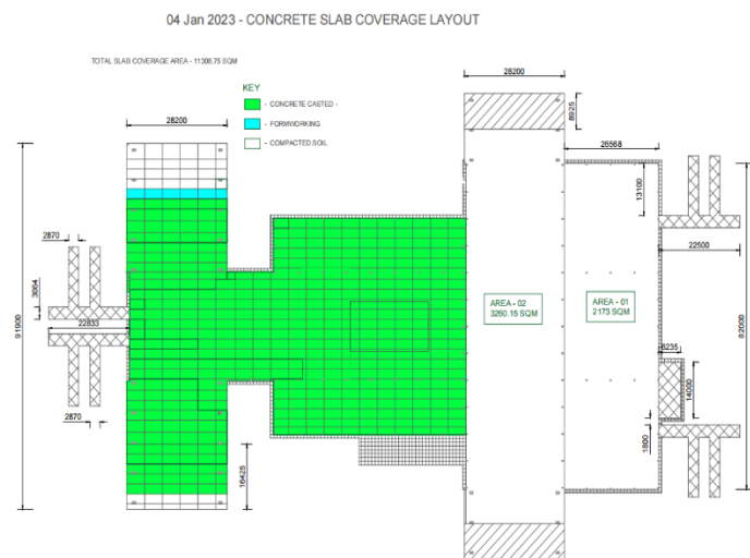
Status of Slab @ Coating Yard
